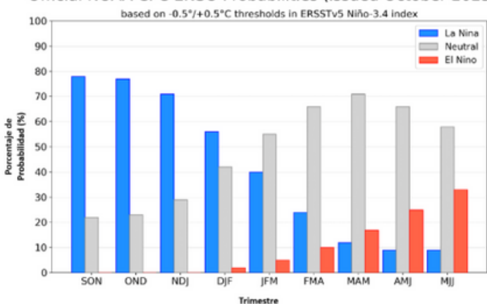
Official NOAA CPC ENSO Probabilities (issued October 2025)
